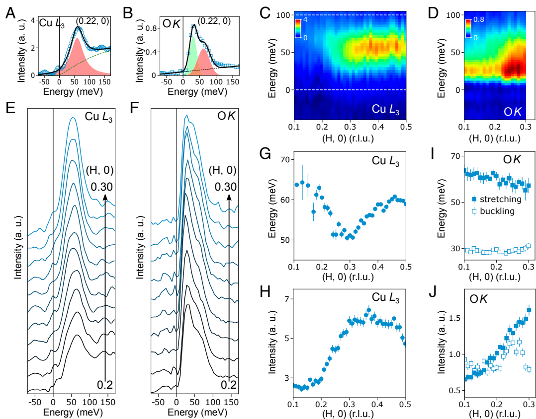
Fig. 2. Phonons in underdoped UD23. (A and B) Fitting examples of the inelastic excitation at the \text{Cu } L_3 - and \text{O } K edges. Fitting details are described in Materials and Methods . (C and D) \text{Cu } L_3 - and \text{O } K RIXS intensity maps as shown in Fig. 1 C and D with the fitted elastic peak subtracted. (E and F) \text{Cu } L_3 - and \text{O } K RIXS spectra after removing the fitted elastic peaks at selected momentum transfer values ranging from q_{\parallel} = 0.2 to 0.3 r.l.u. along the (H, 0) direction. (G and H) The fitted dispersion and the integrated intensity of the bond-stretching phonon excitations at the \text{Cu } L_3 edge as a function of momentum. The phonon spectral weight is integrated within the energy window (0–100 meV) illustrated by the white dotted line in C. (I and J) The dispersion and integrated intensity of the bond-buckling phonon (the high-energy peak, filled markers) and the bond-buckling phonon (the low-energy peak, open markers) at the \text{O } K edge. The dispersion is extracted from the fitting. Phonon intensity is the area of the curve fitting each phonon mode.
